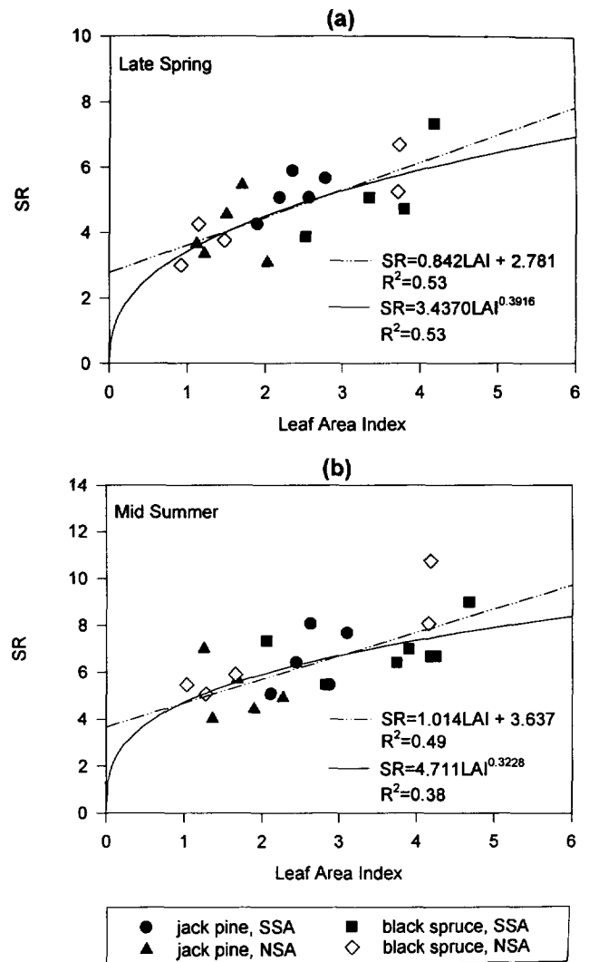
Figure 2. Relationships between SR and LAI in a) late spring and b) mid-summer. SR is calculated from the surface NDVI shown in Figure 1.
