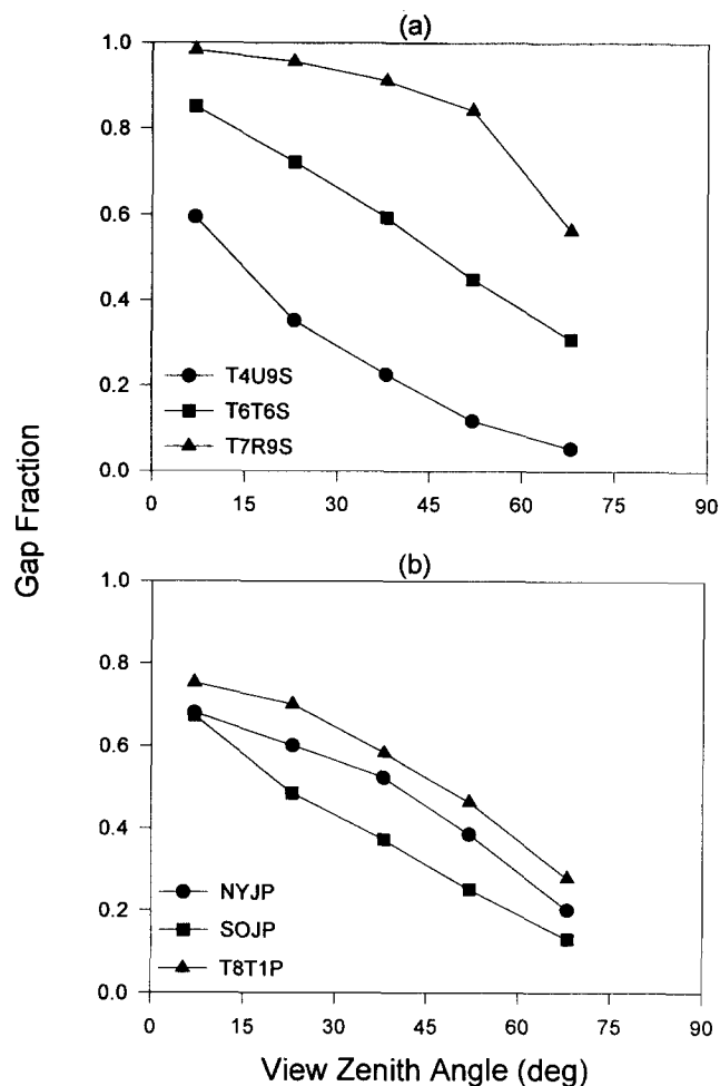
Figure 5. Gap fraction angular distribution patterns for a) black spruce stands and b) jack pine stands.
