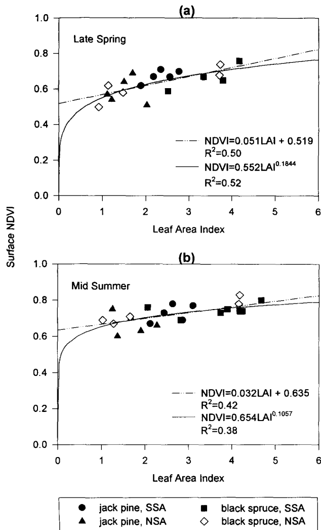
Figure 1. Relationships between NDVI and LAI for boreal conifer forests in a) late spring and b) mid-summer. The surface NDVI is calculated from Landsat TM Band 3 (red) and Band 4 (near-infrared) reflectances at the surface level after atmospheric corrections. The LAI is obtained based on optical measurements with considerations for the foliage clumping and the contributions from the supporting woody material.
