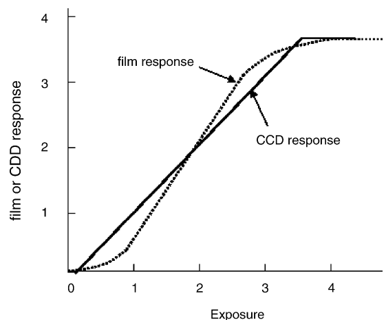
Fig. 1. Schematic diagram for characteristic curves of the response of digital and film media to exposure (both axes are on logarithmic scales).
