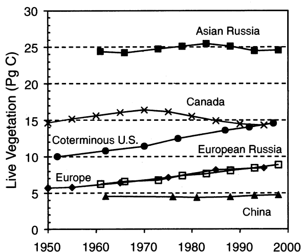
FIG. 1. Carbon stocks in live forest vegetation over the last half century in Canada (Kurz and Apps 1999), the coterminous United States (Birdsey and Heath 1995), Europe (G.-J. Nabuurs, A. Pussinen, M.-J. Schelhaas, and G. M. J. Mohren, unpublished manuscript ), Russia (Shvidenko and Nilsson, in press ), and China (Fang et al. 2001).
