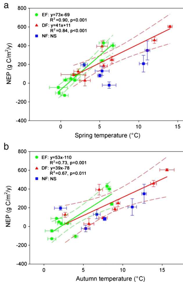
Fig. 8. Relationships between annual NEP (a) spring, (b) autumn temperature for evergreen forest (EF), deciduous forest (DF), and non-forest (NF) sites. Points represent data ( \pm standard error) for each site.
