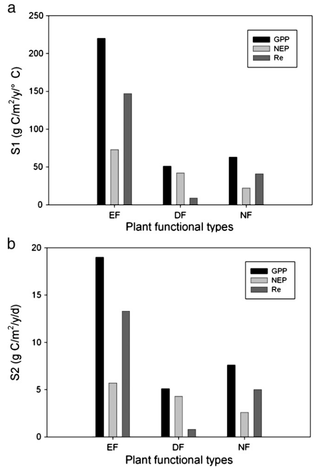
Fig. 11. Sensitivity of ecosystem carbon fluxes (GPP, NEP and Re) to (a) spring temperature and (b) growing season length. S1 ( \text{g C/m}^2/\text{y}/^\circ \text{C} ) is the slope of the correlation between C fluxes and spring temperature and S2 ( \text{g C/m}^2/\text{y}/\text{day} ) is the slope of the correlation between C fluxes and GSL. EF, DF and NF represent evergreen forests, deciduous forests, and non-forest sites, respectively.
