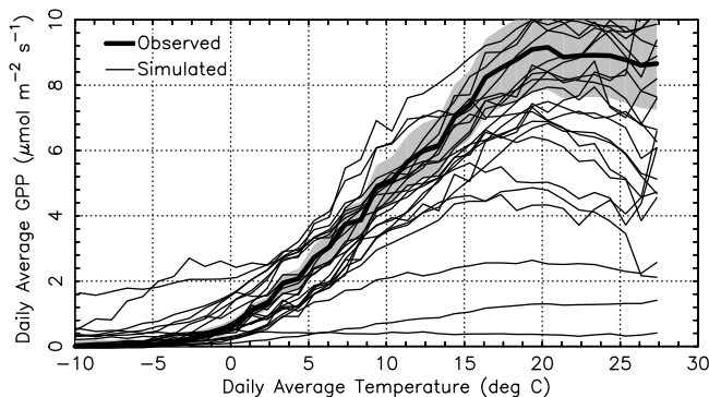
Figure 8. The temperature response curve for US-Ho1 showing simulated and observed GPP as a function of daily mean air temperature. US-Ho1 is the site closest to the average response for all sites. The gray bar indicates uncertainty in the observed GPP response to air temperature.
