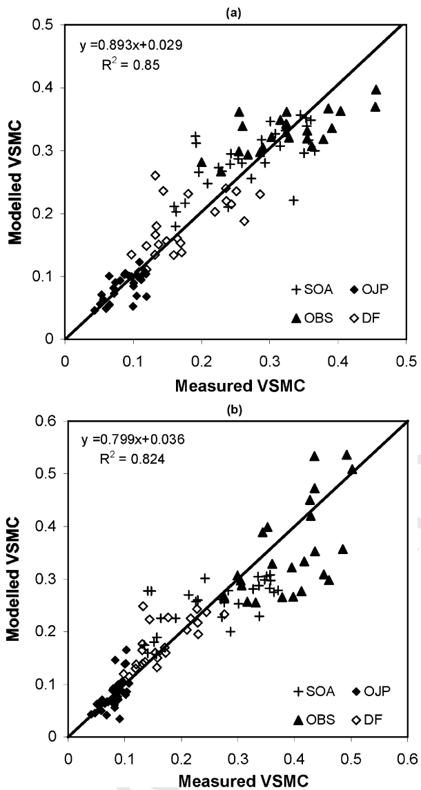
Fig. 2. Comparison of modelled monthly mean volumetric soil moisture content (VSMC) with measurements in the growing season (May to October) at four tower-flux sites: (a) 0–10 cm; (b) 10–30 cm. All measurements of VSMC were interpolated or extrapolated and then averaged to values in the 0–10 cm and 10–30 cm depths. SOA: 75-yr-old aspen site, Saskatchewan; SOBS: 121-yr-old black spruce site, Saskatchewan; SOJP: 65-yr-old jack pine site, Saskatchewan; and DF: 53-yr-old Douglas-fir site, Vancouver Island, BC. The straight solid line is the 1:1 line.
