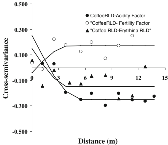
Fig. 5 Cross-semivariograms between coffee ( Coffea arabica ) fine root length (RLD) and Erythrina poeppigiana RLD, and soil factors
