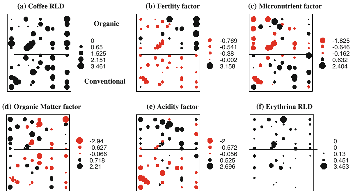
Fig. 2 Bubble plots for coffee fine root density (RLD, \text{cm cm}^{-3} ), Erythrina poeppigiana RLD, and soil factor scores for different locations in the Coffea arabica - Erythrina
