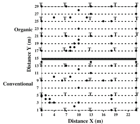
Fig. 1 Sampling scheme in organic and conventional plots of the Coffea arabica - Erythrina poeppigiana association. Black dots, dash, and, “T” denote sample cores, coffee rows, and, the location of E. poeppigiana trees, respectively
