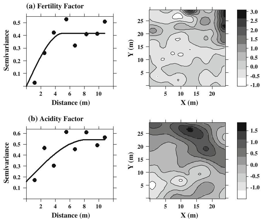
Fig. 4 Semivariograms of soil factors extracted by factorial analysis ( left ). Kriged maps for soil factor scores estimated across the organic and conventional plots ( right ). In kriged maps, above 15 m on the Y axis represents the organic plot, below the conventional plot
