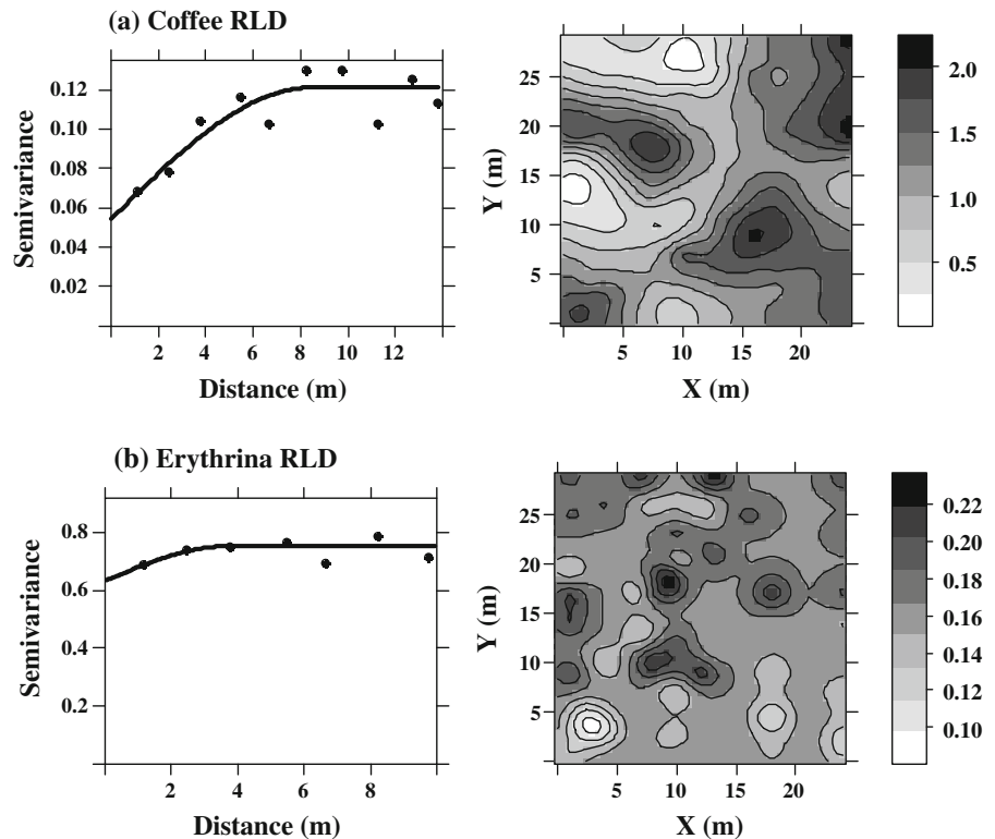
Fig. 3 Semivariograms of residuals from the linear model of density of coffee fine root length (RLD, \text{cm cm}^{-3} ) on soil factors extracted by factorial analysis ( left ). Kriged maps for coffee RLD and Erythrina RLD estimated across the organic and conventional plots ( right ). In kriged maps, above 15 m on the Y axis represents the organic plot, below the conventional plot
